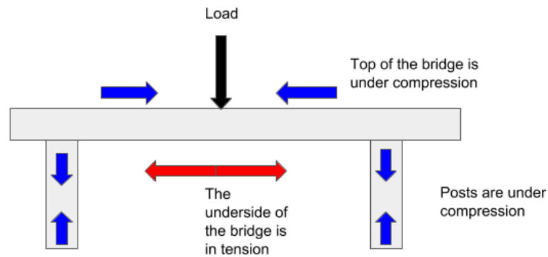
Post and Beam Bridge
